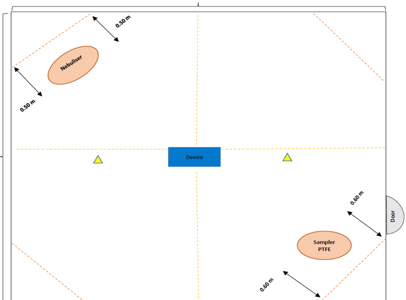
Figure 1 Illustration of the test room (height: 2.4 m) and the positioning of the, nebuliser (height: 0.9 m), sampling device (height 1.2) and the AWE 300 (blue shading). Yellow beacons indicate positions where the sound measurements were taken.
